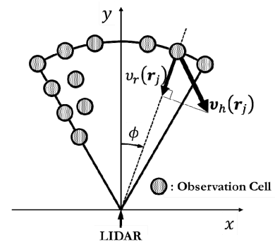
Fig. 1. System model.
