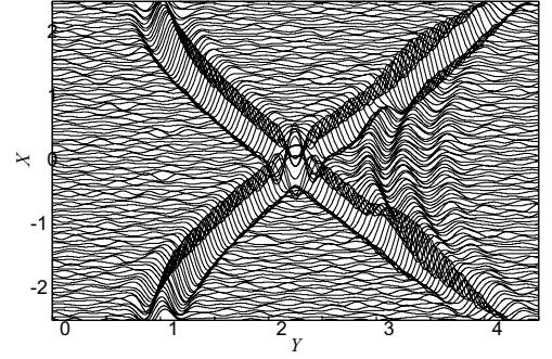
Fig. 11. Output of the matched filter for a concave target.
