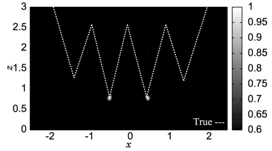
Fig. 4 Estimated image with the conventional SAR algorithm I_1(\mathbf{r}) for the complex-shaped target.
