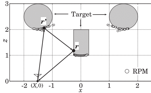
Fig. 3 Target points passed by a double scattered wave and target points with the RPM.
