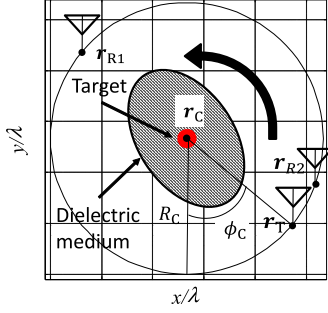
Fig. 1 System model.
