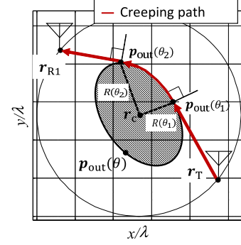
Fig. 2 Propagation path of creeping wave.
