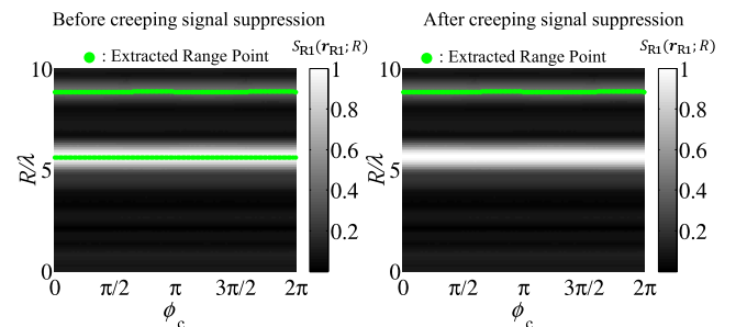
Fig. 4 Outputs of Wiener filter as S_{R1}(\mathbf{r}_{R1}; R) and extracted range points before (left) and after (right) creeping wave suppression.
