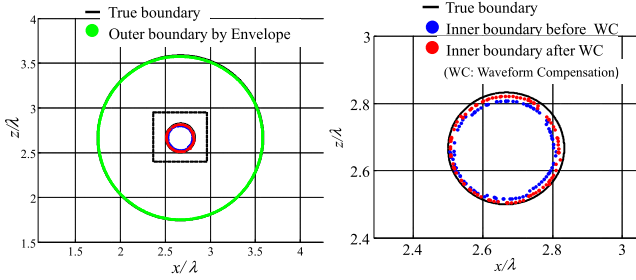
Fig. 6 Actual and reconstructed image before and after waveform compensation (WC) (right: enlarged view for internal object).
