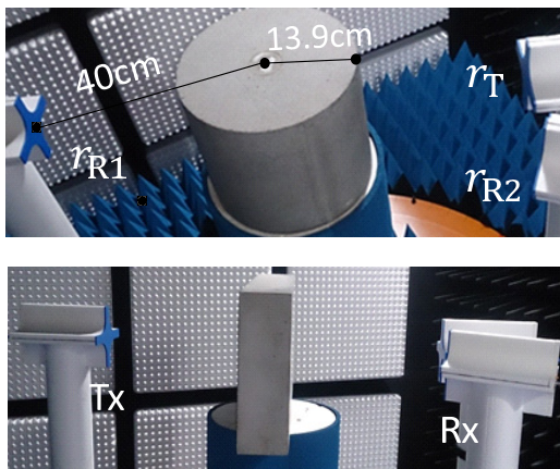
Fig. 3 Setup for the experiment (upper) and setup for obtaining actual dielectric constant of cement object (lower).
