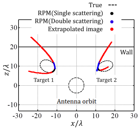
Fig. 4 Extrapolation in real space where single and double scattered signals are used.
