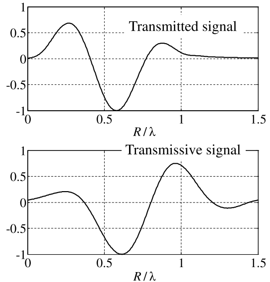
Fig. 4 Transmitted (upper) and transmissive signal waveforms (lower).
