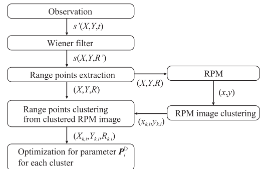
Fig. 4 Flowchart of the proposed method.
