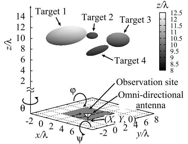
Fig. 17 System model in 3-D problem.
