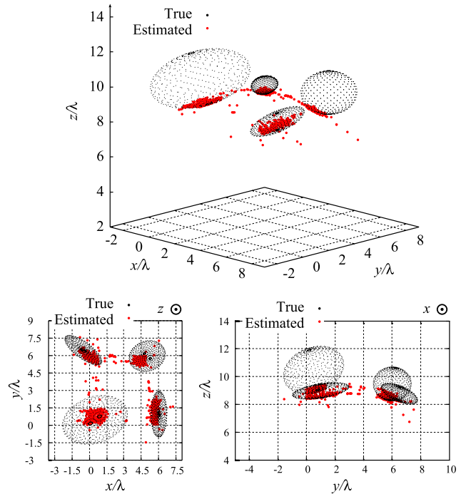
Fig. 18 Estimated target points obtained by the RPM at S/N = 30 dB.
