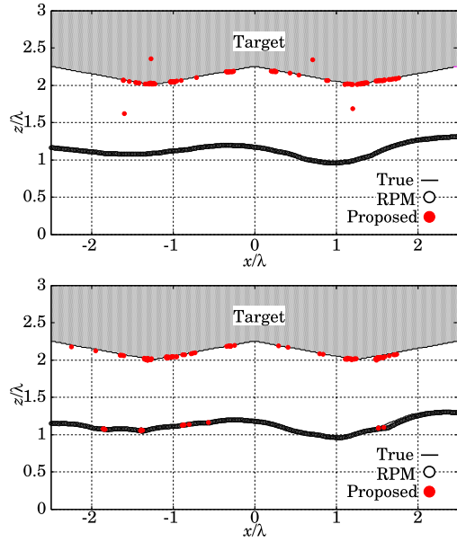
Fig. 11 Estimated image with the proposed algorithm in noisy situation: case (b) (upper: S/N=20 dB, lower: S/N=10 dB).
