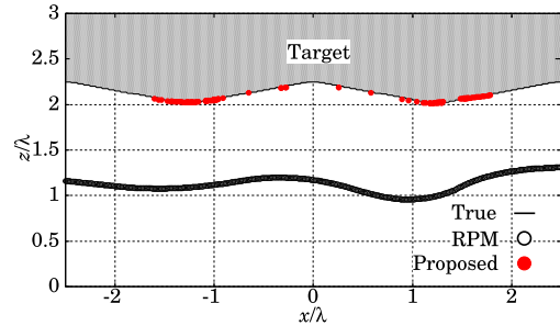
Fig. 10 Estimated image with the proposed algorithm in noiseless situation: case (b).
