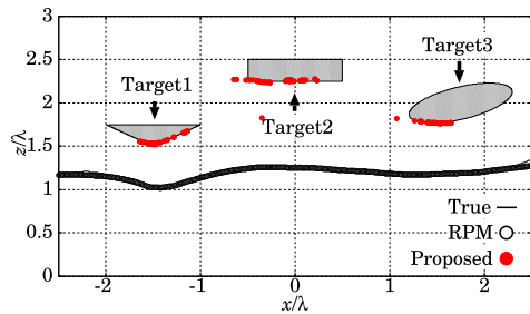
Fig. 16 Estimated image with the proposed algorithm in the inhomogeneous medium in S/N=20 dB:case(a).
