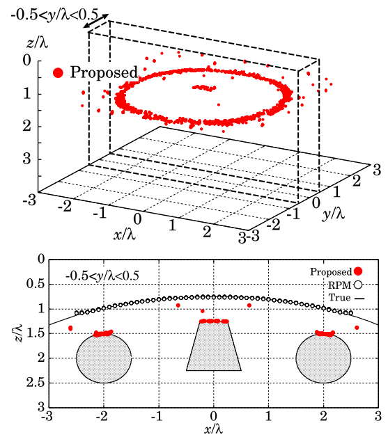
Fig. 22 Estimated target points with the proposed algorithm for the 3-D targets in S/N=25 dB.
