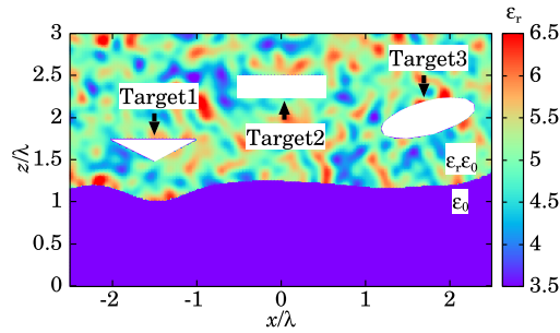
Fig. 15 Relative permittivity distribution in the inhomogeneous medium: case(a).
