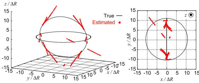
Fig. 22 3-D reconstruction image obtained by the conventional method in the experiment (Case A).
