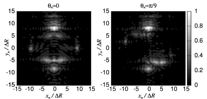
Fig. 21 ISAR images at the rotation angles \theta = 0 (left) and \theta = \pi/9 (right) in the experiment (Case A).
