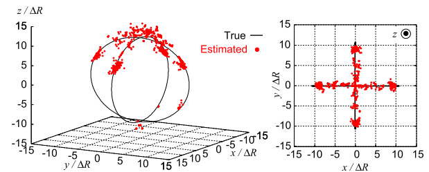
Fig. 27 3-D reconstruction image obtained by the extended RPM method in the experiment (Case B).
