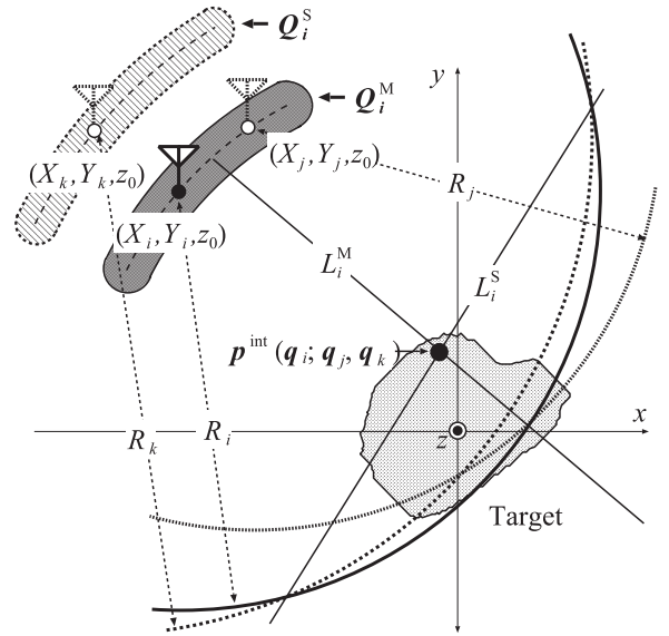
Fig. 11 Relationship among intersection point p^{\text{int}}(q_i; q_j, q_k) , two intersection lines L_i^M and L_i^S and target boundary.
