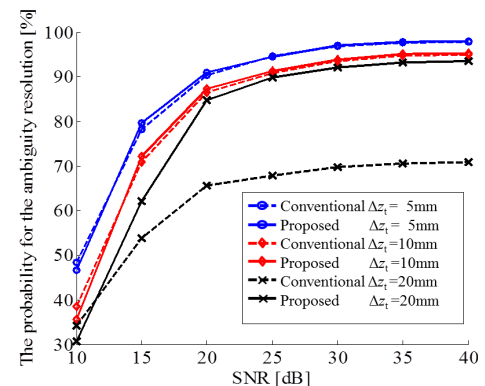
Fig. 11 The probability for the ambiguity resolution in each SNR and height change \Delta z_t .
