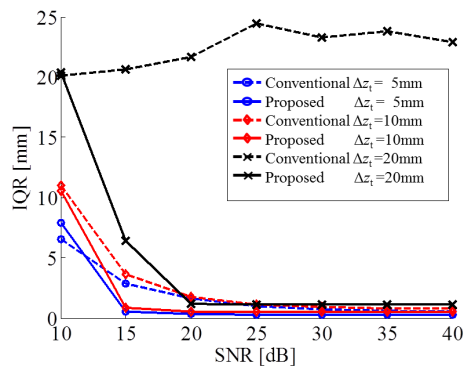
Fig. 13 The inter quartile range in each SNR and height change \Delta z_t .
