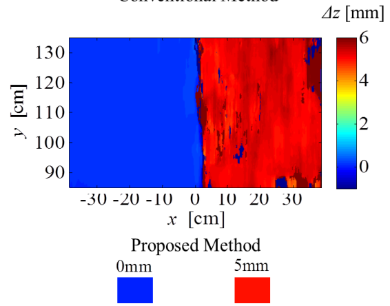
Fig. 16 Estimated distribution of the height change \Delta z_t = 5 mm, obtained by each method in experiment (upper: Conventional, lower: Proposed).
