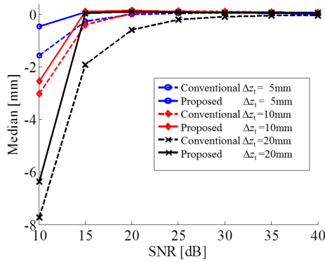
Fig. 12 The median error in each SNR and height change \Delta z_t .
