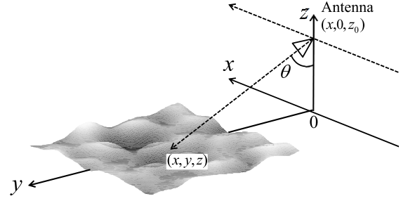
Fig. 1 Observation geometry.
