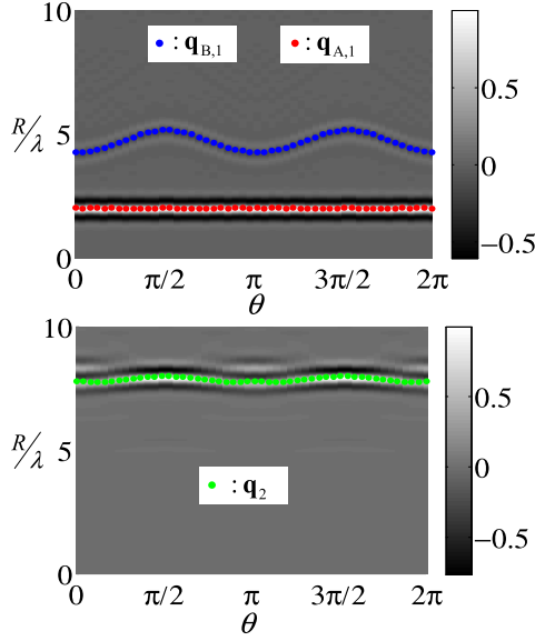
Fig. 7 Outputs of Wiener filter S_1(X, Z, R) (upper) and S_2(X, Z, R) (lower) in Case #1.
