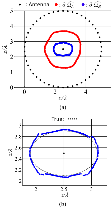
Fig. 10 (a) Estimated dielectric boundaries for \Omega_A and \Omega_B using the proposed method, (b): Enlarged view for \Omega_B in Case #2.
