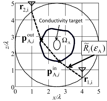
Fig. 2 Propagation path estimation in the conventional method.
