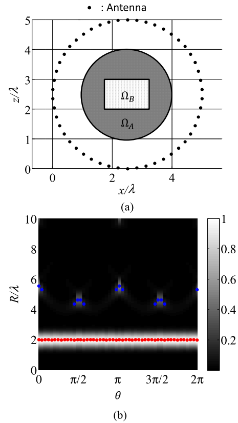
Fig. 11 (a) Actual boundary assuming the rectangular inner object, (b): Output of Wiener filter S_1(X, Z, R) .
