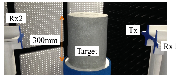
Fig. 12 Experimental setup.
