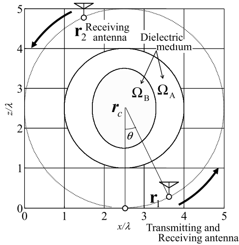
Fig. 1 System and observation model.
