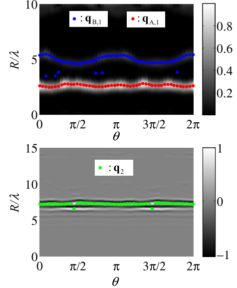
Fig. 9 Outputs of Wiener filter S_1(X, Z, R) (upper) and S_2(X, Z, R) (lower) in Case #2.
