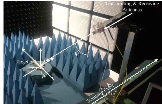
Fig. 3 Experimental setup.
