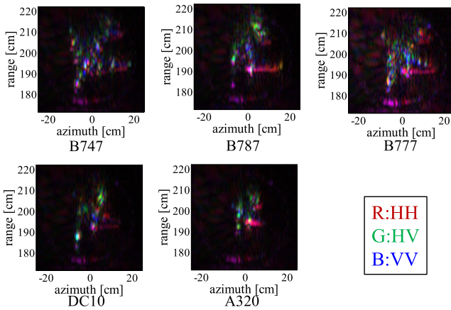
Fig. 8 RGB expression for SAR images on LP basis for each airplane at \phi = 30^\circ .
