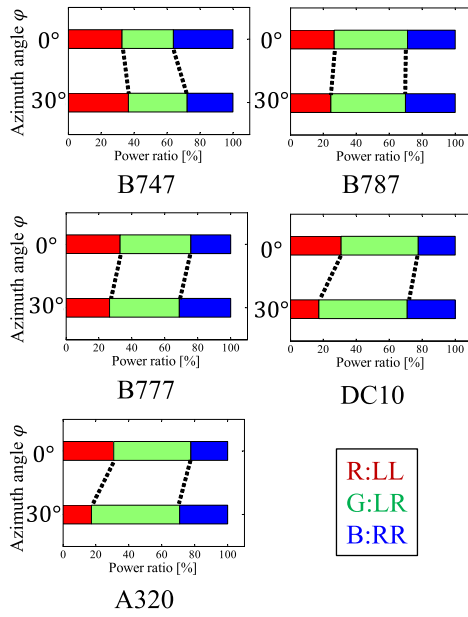
Fig. 12 Power ratio of CP basis in red marked area.
