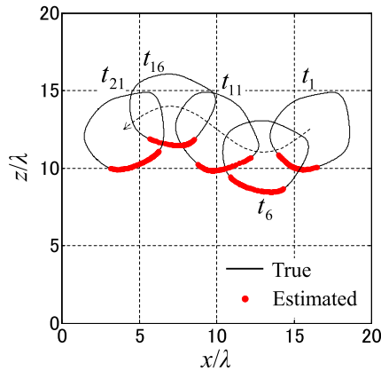
Fig. 9 Target boundary points obtained by multi-static RPM algorithm in noiseless situation at t_1 , t_6 , t_{11} , t_{16} and t_{21} .
