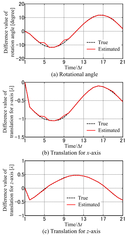
Fig. 20 Target motion for each observation time estimated by the proposed method in considering the target motion during data acquisition time. ((a) Difference value of rotation angle (b) Difference value of translation motion for x-axis (c) Difference value of translation motion for z-axis.)
