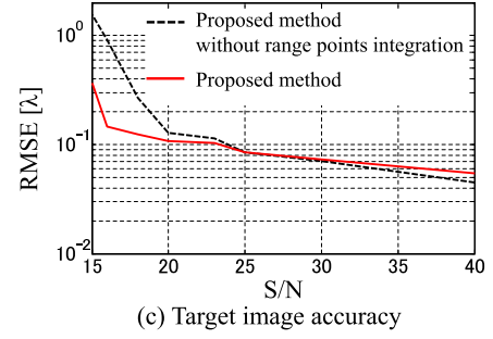
Fig. 19 RMSE in target imaging accuracy versus S/N for the proposed method.
