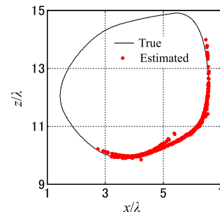
Fig. 16 Reconstructed target image by the proposed method including the range points integration as in Sect. 4.3 in S/N = 20 dB.
