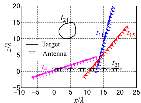
Fig. 12 The compensated locations of antenna from t_4 , t_{11} , t_{15} , and when the target is assumed to be static at the position of t_{21} .
