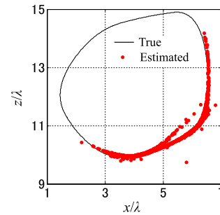
Fig. 15 Reconstructed target image by the proposed method without the range points integration as in Sect. 4.3 in S/N = 20 dB.
