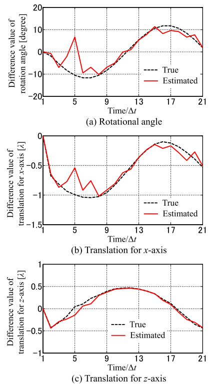
Fig. 14 Target motion for each observation time estimated by the proposed method in S/N = 20 dB. ((a) Difference value of rotation angle (b) Difference value of translation motion for x-axis (c) Difference value of translation motion for z-axis.)
